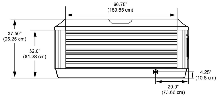
FRONT/BACK VIEW Tolerance: \pm 0.5" (1.27 cm)
