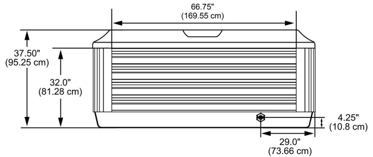
FRONT/BACK VIEW Tolerance: \pm 0.5" (1.27 cm)
